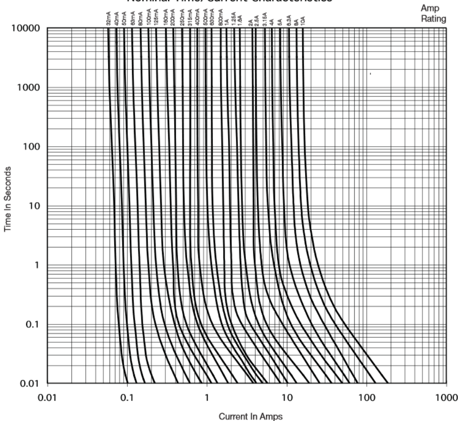
Time-current Curve Nominal Time/Current Characteristics
