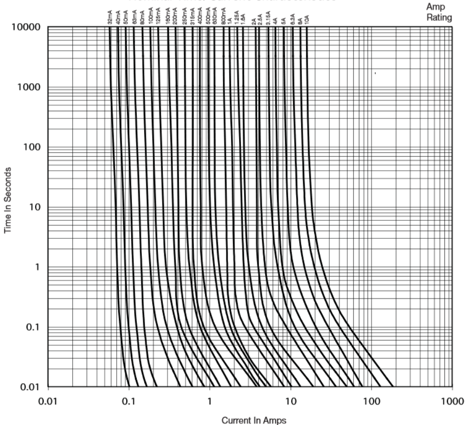
Nominal Time/Current Characteristics
